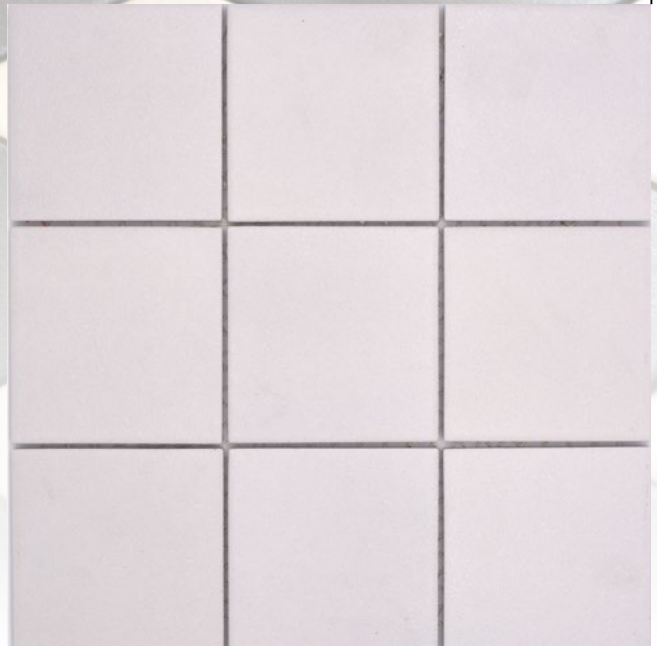
RAT 200 Matte/sheet 298x298mm Stein/stone 97x97x6mm / R10B
